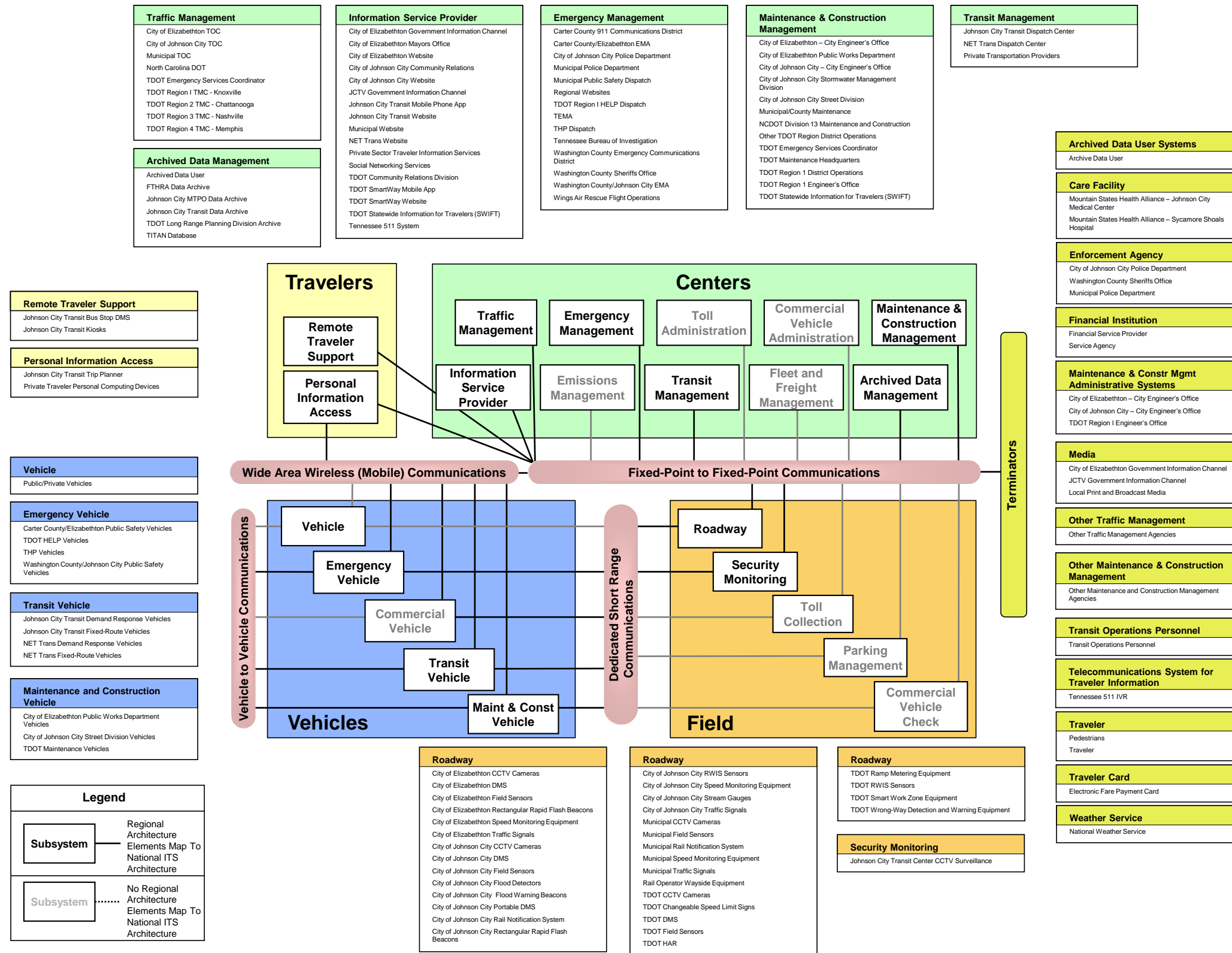
Figure 5 – Johnson City Regional System Interconnect Diagram
